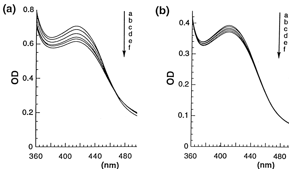
Figure 2. Visible spectra of (a) 4 , and (b) 8 in the presence of calf thymus DNA at 298 K, in 10 mM Tris-HCl buffer (pH 7.0) containing 20% of DMF, [Compound] = 2.1 \times 10^{-5} \text{ M} , [calf thymus DNA] = (a) 0, (b) 1.6 \times 10^{-5} , (c) 3.2 \times 10^{-5} , (d) 4.8 \times 10^{-5} , (e) 6.4 \times 10^{-5} , (f) 8.0 \times 10^{-5} \text{ M} .
