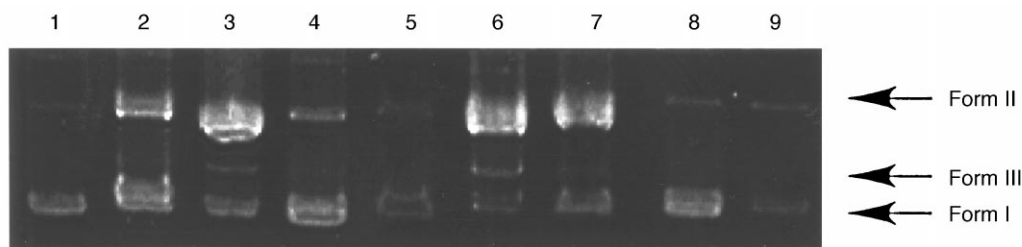
Figure 3. Agarose gel electrophoresis patterns of plasmid pBR322 DNA after treatment of reductively activated nitro 5-deazaflavin derivatives 1–8 . Lane 1–9: Control, 8 , 7 , 6 , 5 , 4 , 3 , 2 , 1 . (The reductive activations of the compounds 1–8 were carried out at a constant potential of -0.95 V versus an aqueous Ag/AgCl under N_2 in 1.5 mM sodium citrate buffer (pH 7.0) containing 25% of DMF). [Compound] = 1.0 \times 10^{-3} (M), [DNA] = 5.0 \times 10^{-5} (M/base pair).
