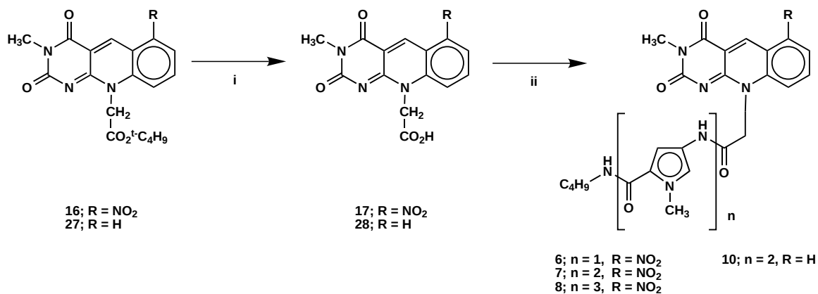
Scheme 4. Synthesis of compounds 6–8 and 10: 1) 12N HCl, 60 °C; ii) 18b–20b, 1,3-Diisopropylcarbodiimide, CH 3 CN or DMF, rt.
