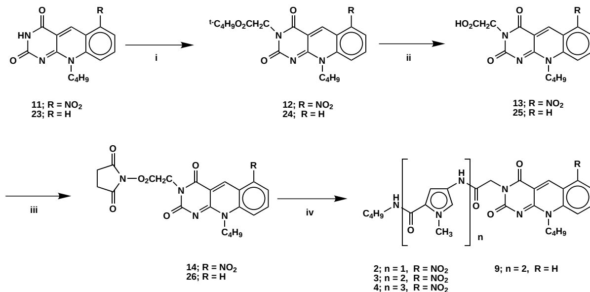
Scheme 2. Synthesis of compounds 2–4, and 9: i) tert -butyl bromoacetate, K 2 CO 3 , DMF, 60 °C; ii) 12N HCl, 60 °C; iii) N,N' -Di-succinimidyl carbonate, Pyridine, CH 3 CN, rt; iv) 18b–20b, DMAP, CH 3 CN, rt.
