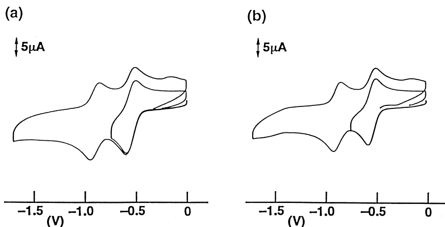
Figure 1. Cyclic Voltammograms of compounds 4 (a) and 8 (b) at 298 K in DMF, [Compound] = 1.0 \times 10^{-3} (M), [\text{Bu}_4\text{NClO}_4] = 1.0 \times 10^{-1} (M) versus an aqueous Ag/AgCl reference electrode under \text{N}_2 .
